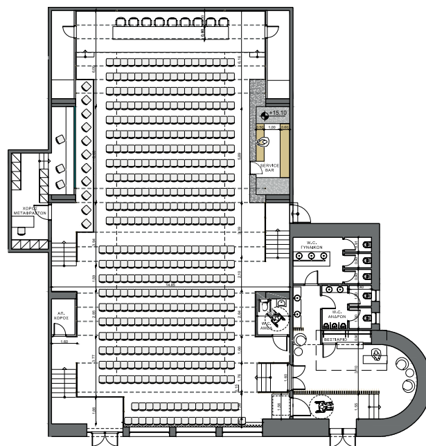
ZEUS CONFERENCE HALL 424.7 m2 h= 3.70
